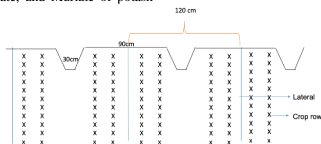
Fig. 1. Schematic representation of Raised bed system.
