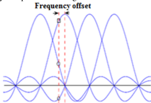
Fig. 2. ICI due to CFO in the OFDM spectrum.
