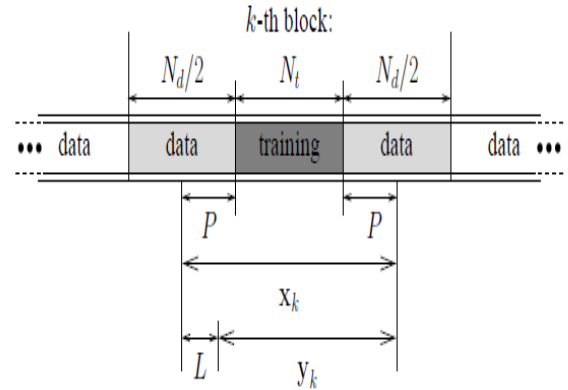
Fig. 1. Partitioning of the transmitted symbol vectors into blocks, each consisting of N_t training and N_d data symbol vectors.
