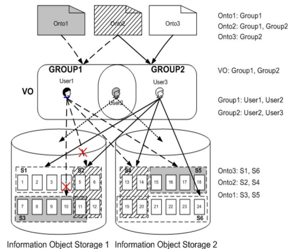
Fig. 2. Access control relation among various ontologies .
