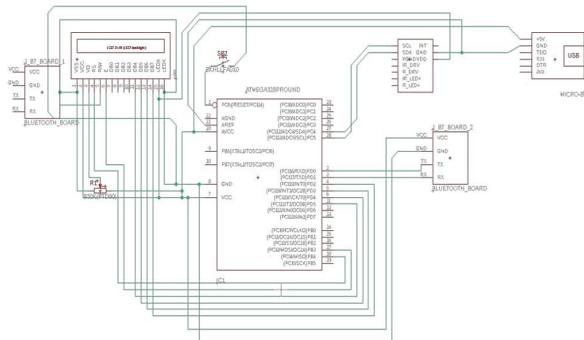
Fig. 5. Schematic Diagram of Device.
